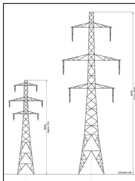
Figure 3 - L7 and L8 tower comparison [source: https://www.ssen-transmission.co.uk/media/2432/ssen-lairg-project-a4-12pp-web-hres.pdf ]
